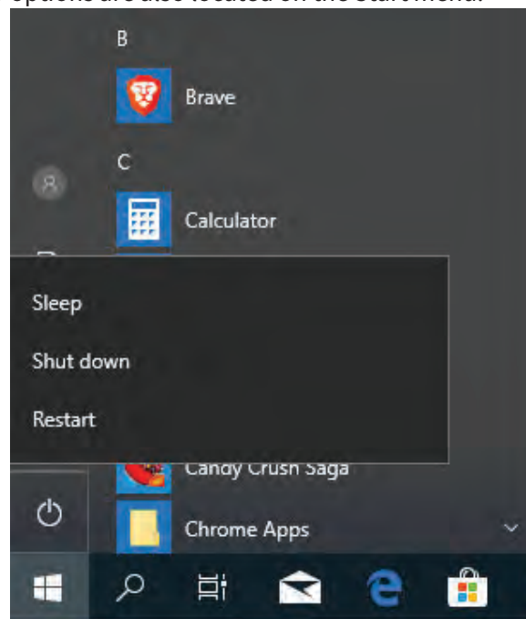
Figure 2.4: Start menu
